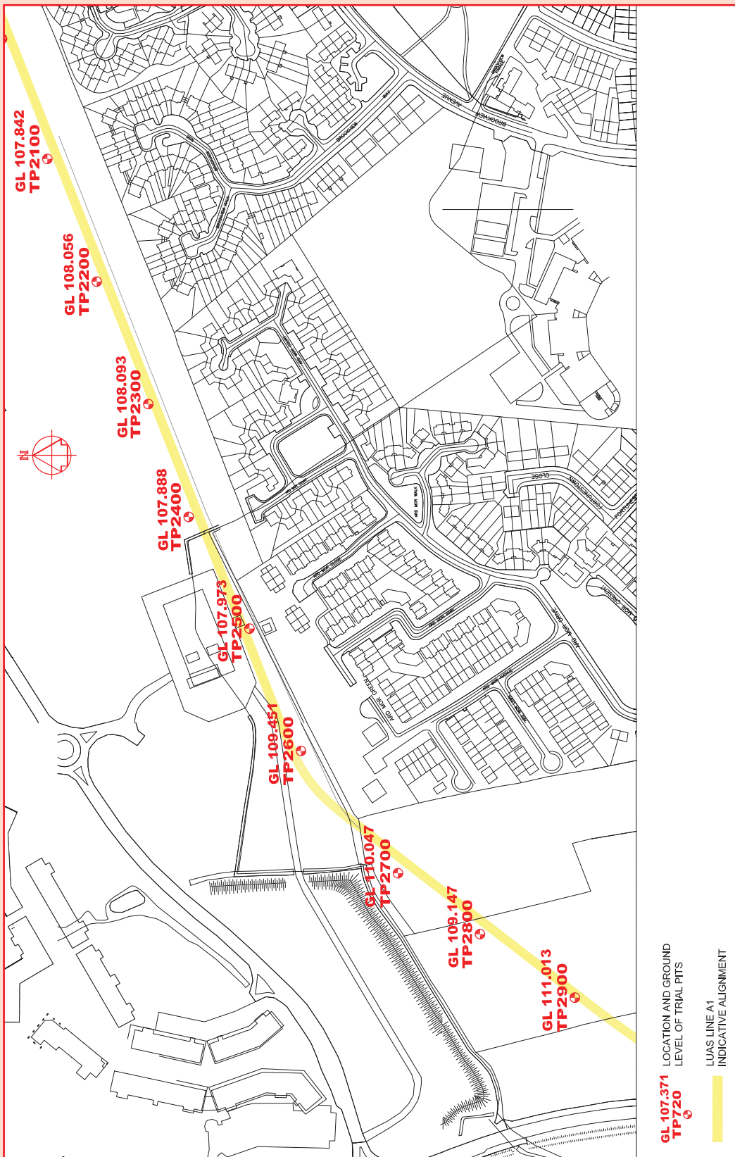
Figure 8.3: Location of Trial Pits (CH 1910.000 to 2840.000)
