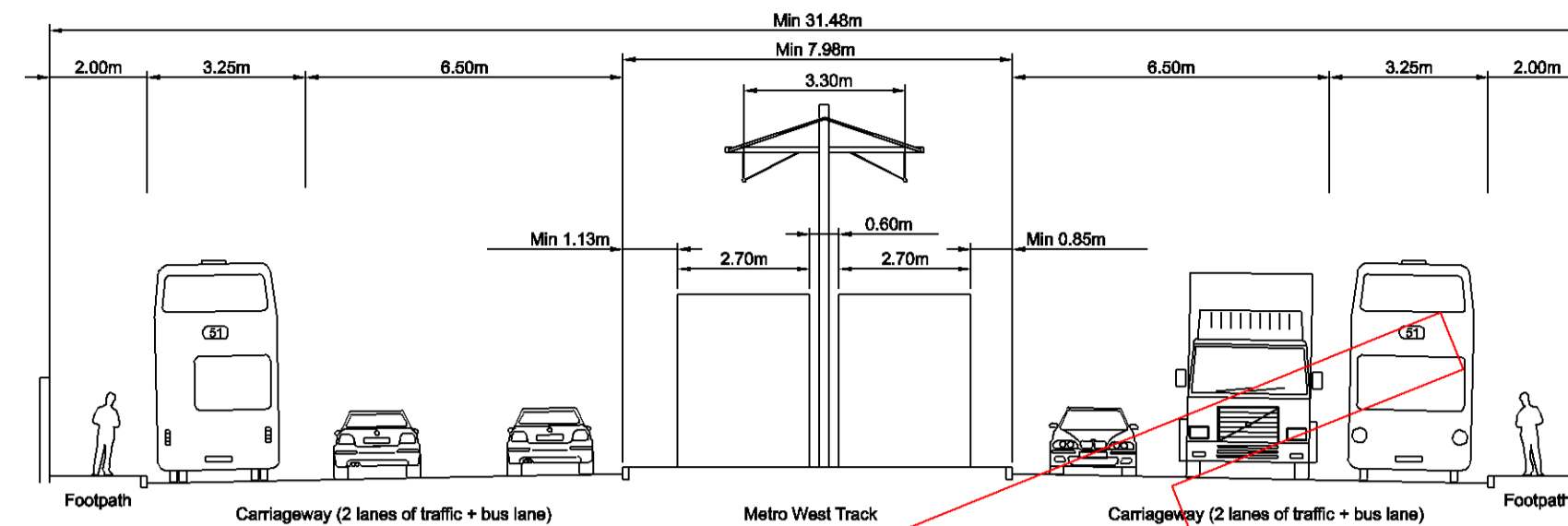
TYPICAL CROSS SECTION AT A-A NOT TO SCALE
